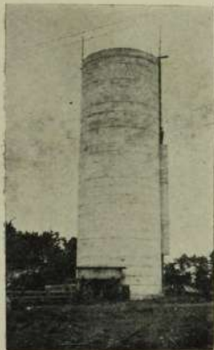
SOLID CONCRETE SILO. Owned by W. J. Beedles, seven miles southeast of Roscoe, Kansas. This silo is 62 feet high and 20 feet in diameter and has a capacity of 502 tons.
